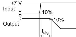
Response Waveform
