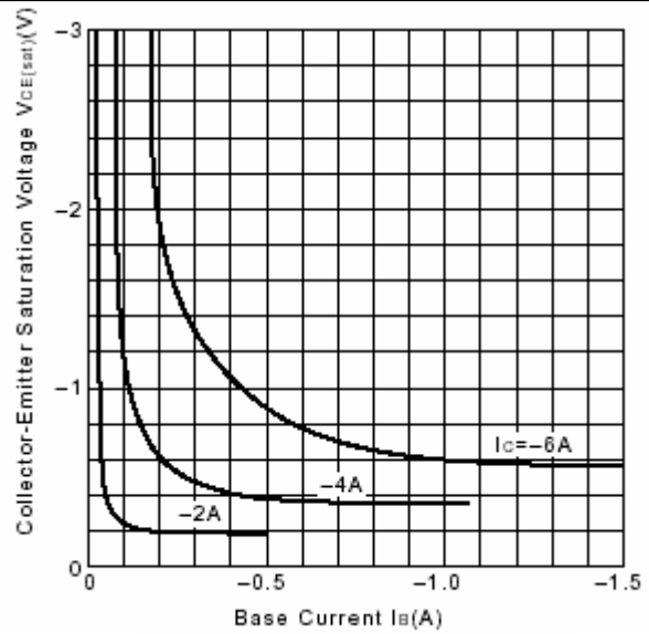
Fig.4 V_{CE(sat)}-I_B Characteristics
